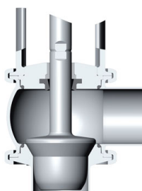
Equal percentage regulating plug
